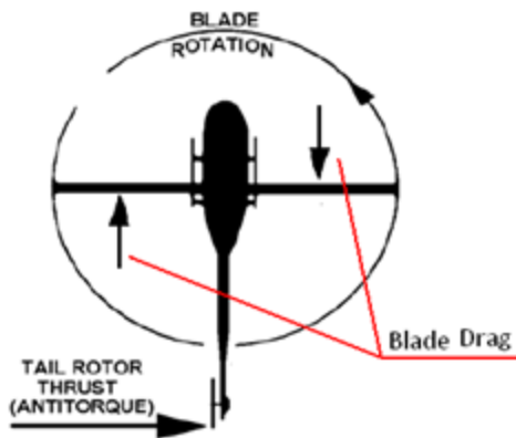
Conventional Helicopter
